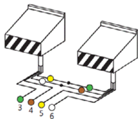
2 x 2-wire cable
